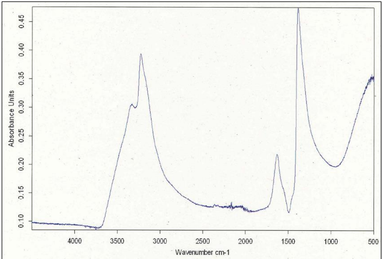
Figure 1. IR spectrum of Diammonium hexachloroplatinate
