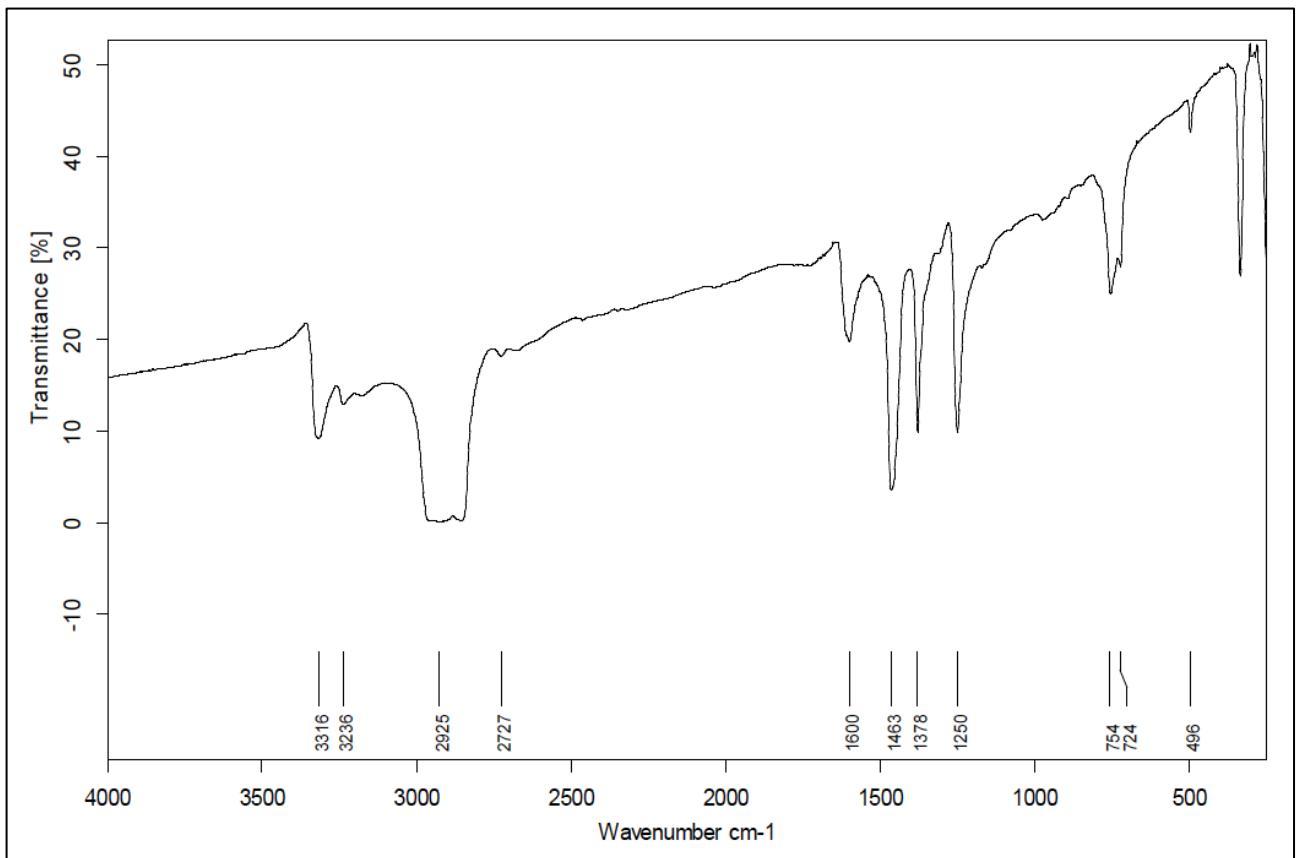
Figure 1. IR spectrum of Diamminedichloropalladium
