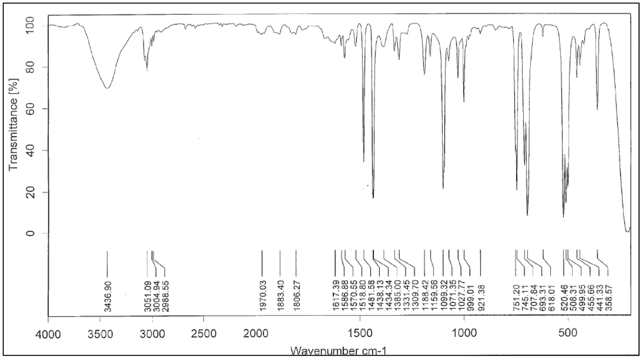
Figure 1. IR spectrum of Dichlorobis(triphenylphosphine)palladium
