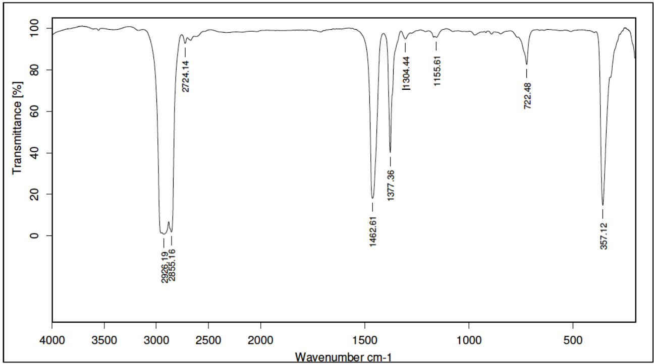
Figure 1. Typical infrared spectrum of dipotassium hexachloropalladate
