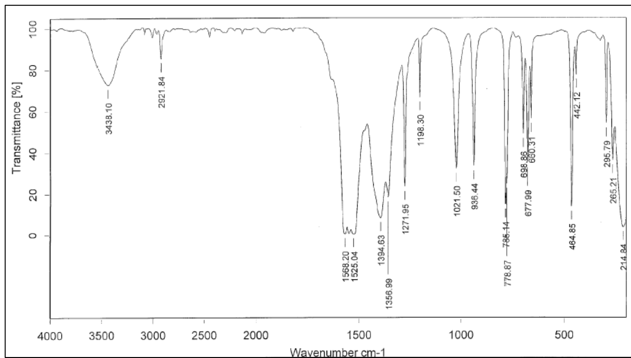
Figure 1. IR spectrum of Palladium (II) di(4-oxopent-2-en-2-oate)
