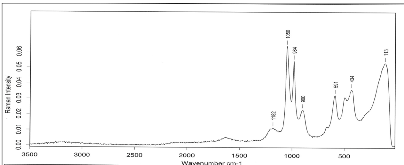
Figure 1. Raman spectrum of Palladium sulphate (solution)
