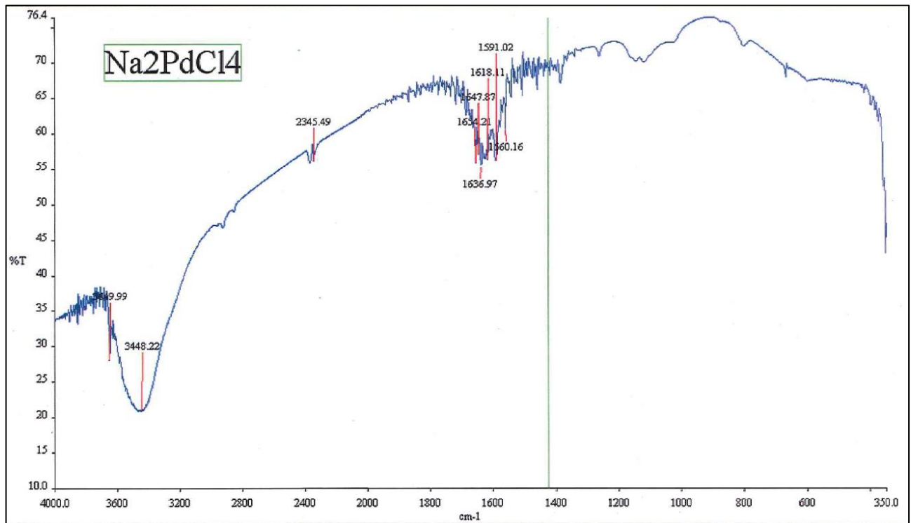
Figure 1. IR spectrum of Disodium tetrachloropalladate
