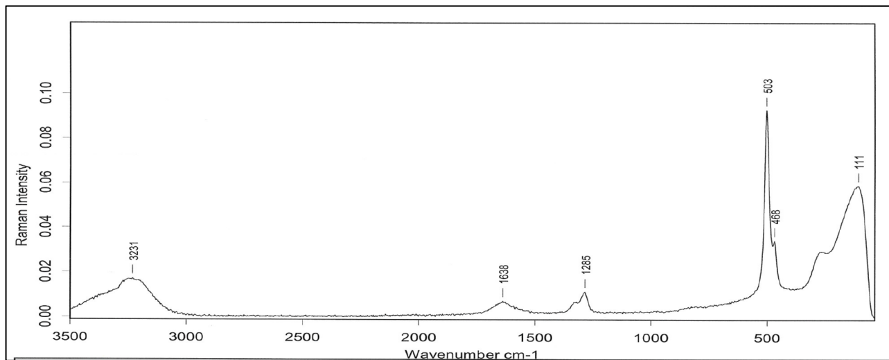
Figure 3. Raman spectrum of Tetraamminepalladium(2+) dichloride solution
