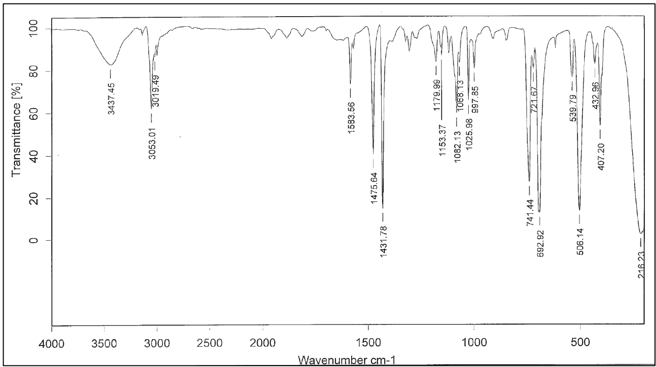
Figure 1. IR spectrum of Tetrakis(triphenylphosphine)palladium
