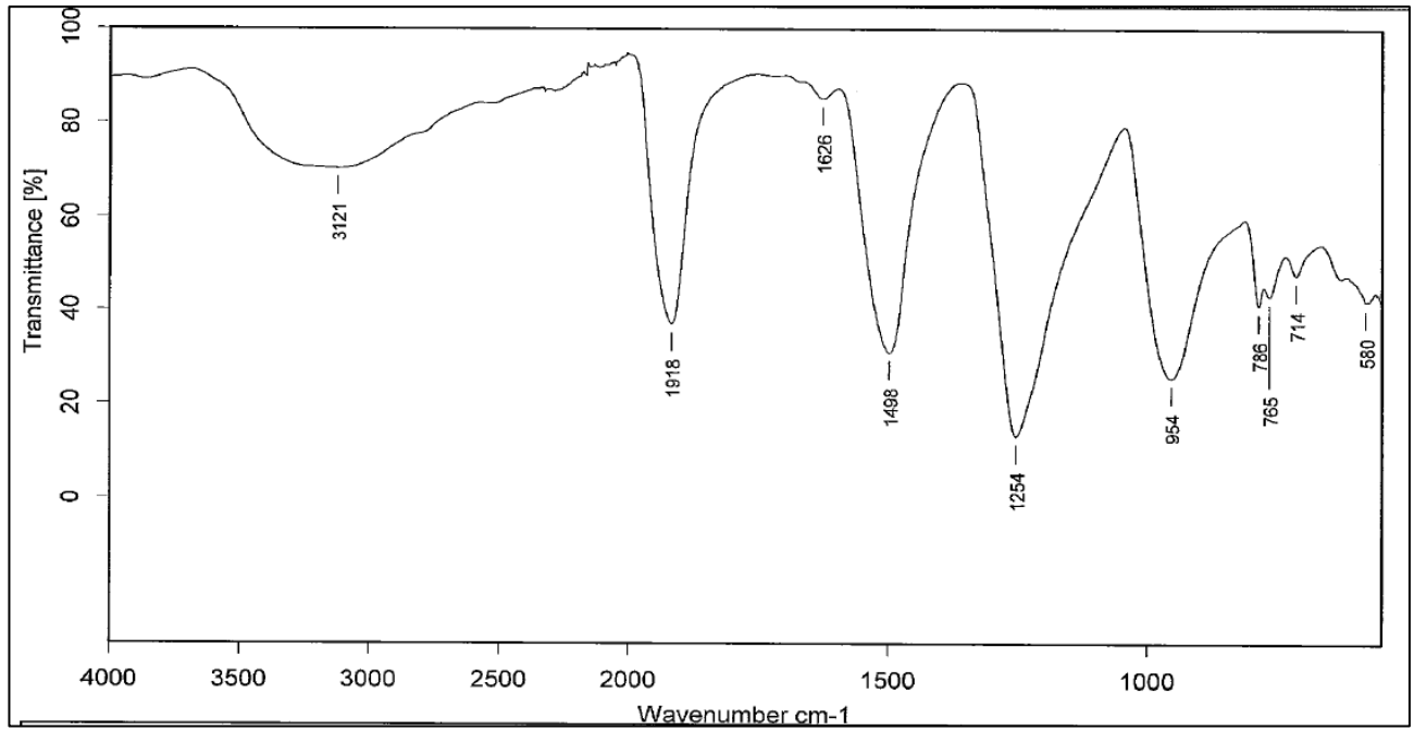
Figure 1. IR spectrum of Tris(nitrato-O)nitrosylruthenium
