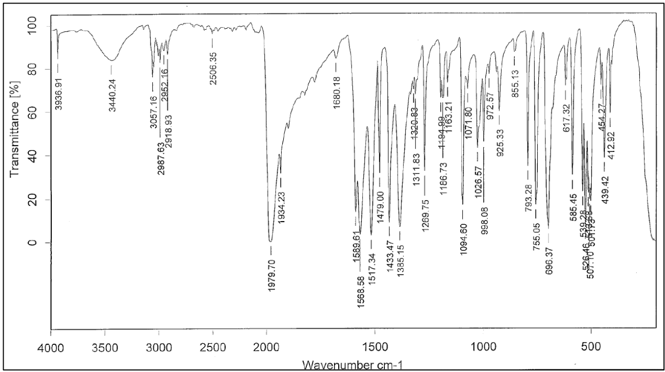
Figure 1. IR spectrum of Carbonyl(pentane-2,4-dionato-O,O')(triphenylphosphine)rhodium
