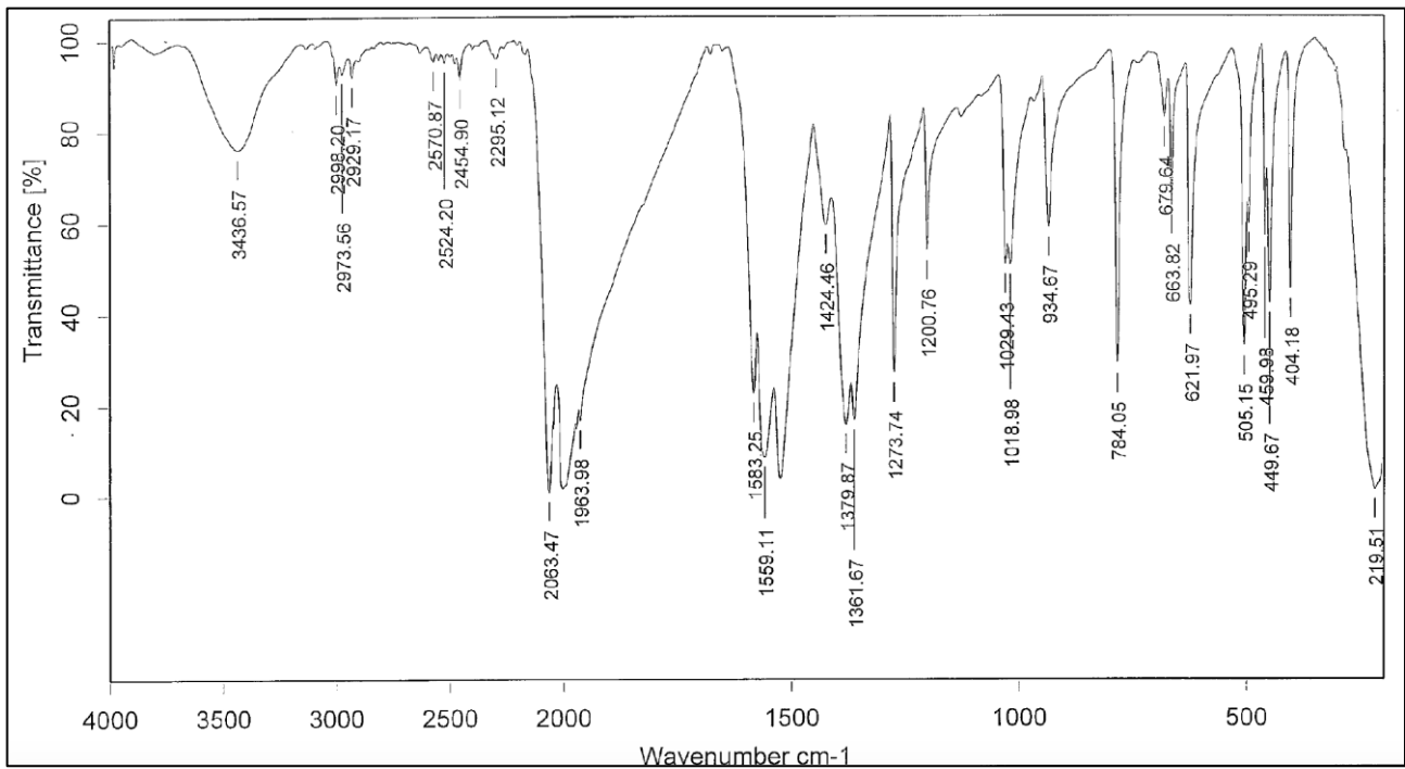
Figure 1. IR spectrum of Dicarbonyl(pentane-2,4-dionato-O,O')rhodium
