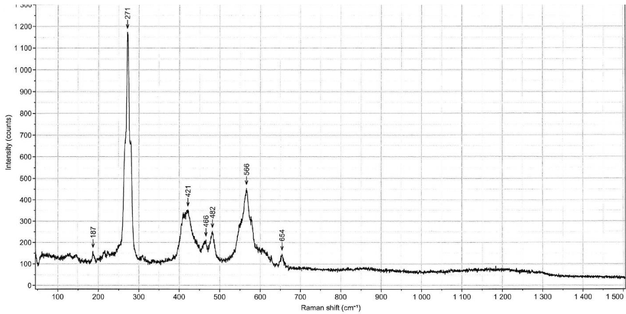
Figure 1. Raman spectrum of Rhodium triiodide
