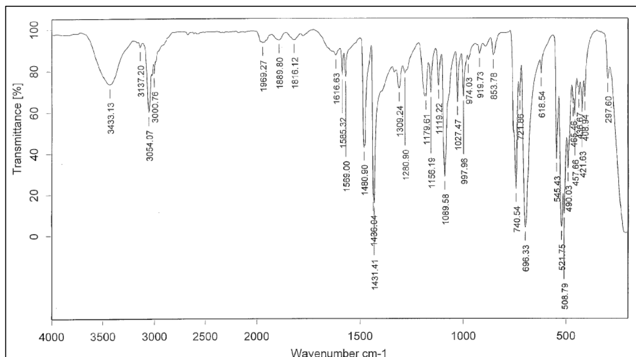
Figure 1. IR spectrum of Tris(triphenylphosphine) rhodium (I) chloride
