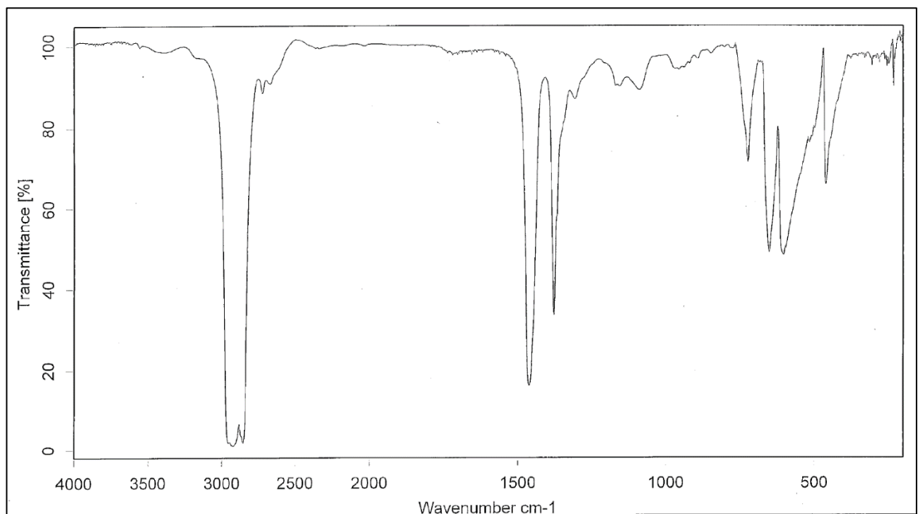
Figure 1. IR spectrum of Dirhodium trioxide
