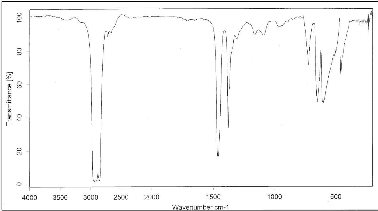
Figure 1. IR spectrum of Dirhodium trioxide
